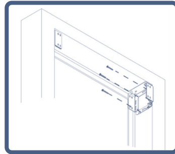
Inside Mount
